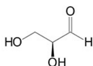
L-Glyceraldehyde
