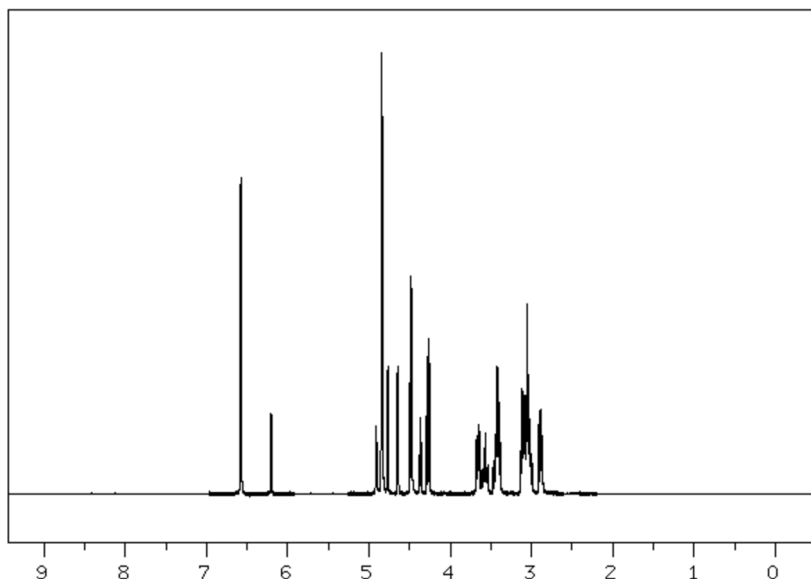
D-glucopyranose
